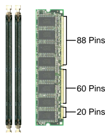
P4SGX-MX 168-Pin DIMM Sockets
