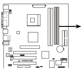
P4SGX-MX 168-Pin DIMM Sockets
