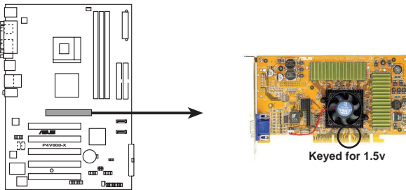
P4V800-X Accelerated Graphics Port (AGP)
