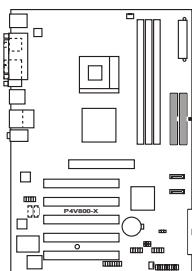
P4V800-X IDE Connectors
