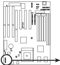
System Panel Connectors
