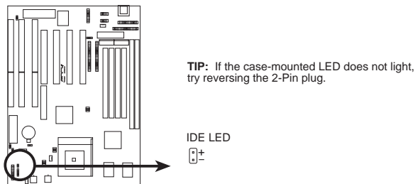
IDE (Hard Drive) LED Lead
