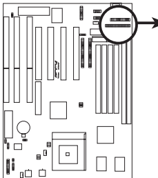
Floppy Drive Connector
