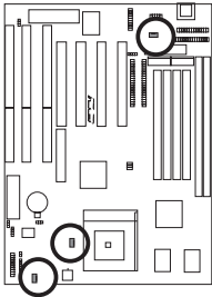
12Volt Chassis, CPU, Power Supply Fan Power
