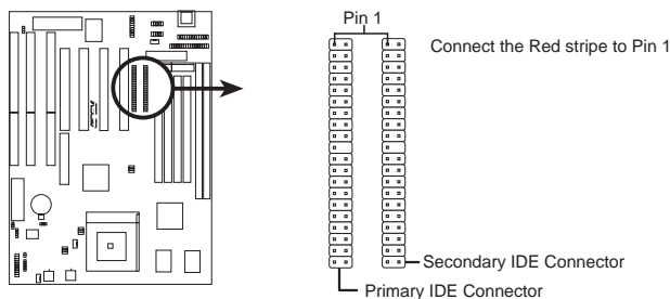
IDE (Hard Disk Drive) Connectors
