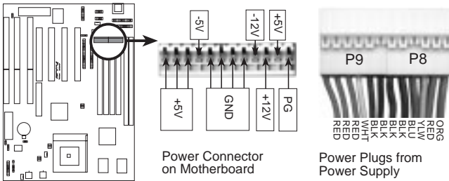
AT Power Connector
