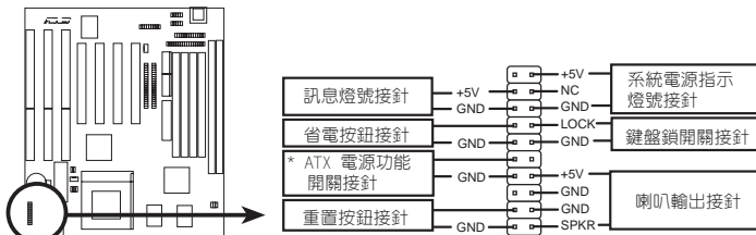
System Panel Connectors
