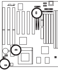
Power Supply, CPU, 12-Volt Chassis Fan Power
