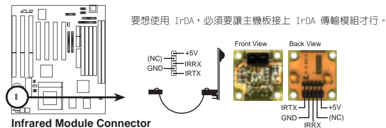
Infrared Module Connector
