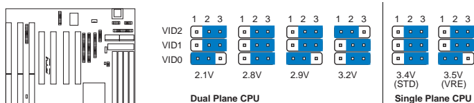
CPU Vcore Voltage ID Selection
