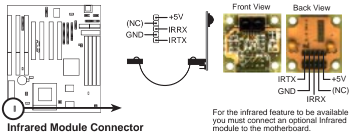
Infrared Module Connector
