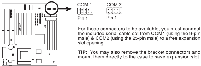
Serial Port Connectors
