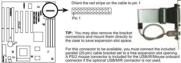
Parallel Port Connector
