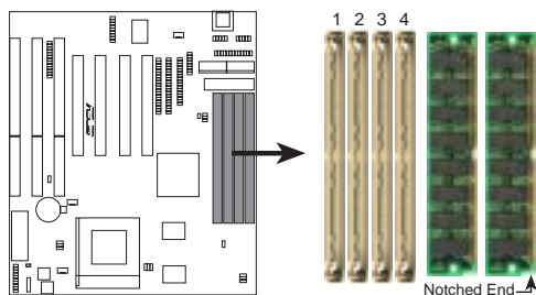
72-Pin SIMM Sockets
