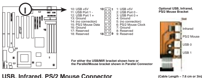
USB, Infrared, PS/2 Mouse Connector
