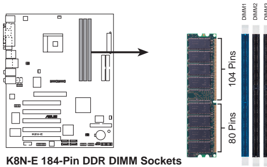
K8N-E 184-Pin DDR DIMM Sockets
