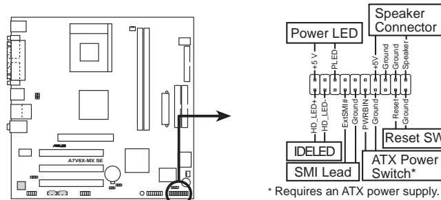
A7V8X-MX SE System Panel Connectors
