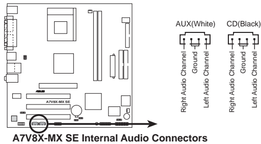
A7V8X-MX SE Internal Audio Connectors
