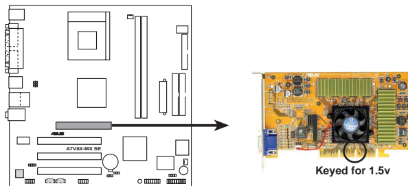
A7V8X-MX SE Accelerated Graphics Port (AGP)
