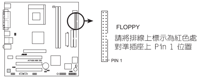
A7V8X-MX SE Floppy Disk Drive Connector
