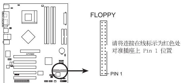
A7V880 Floppy Disk Drive Connector
