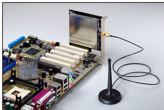
A7V880 WIRELESS Connectors
