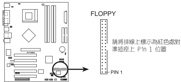
A7V880 Floppy Disk Drive Connector
