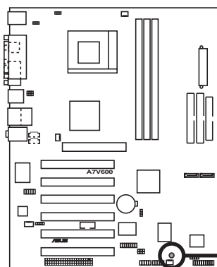
A7V600 Onboard LED
