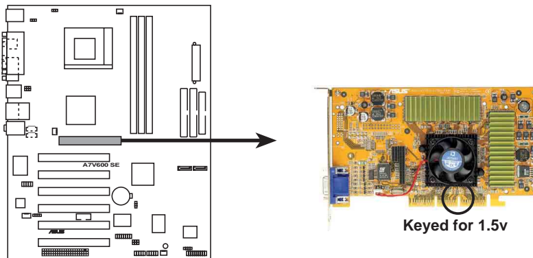
A7V600 SE Accelerated Graphics Port (AGP)
