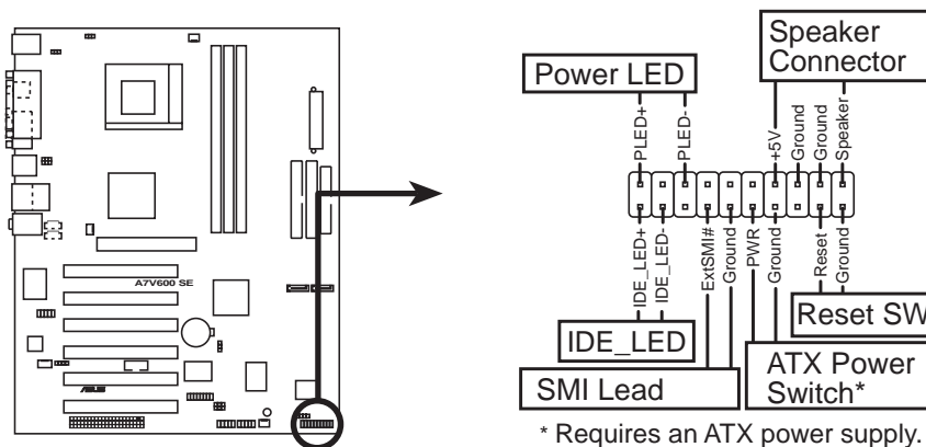
A7V600 SE System Panel Connectors
