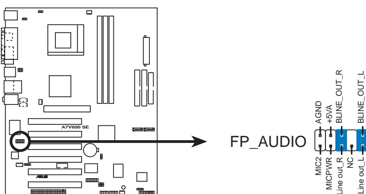
A7V600 SE Front Panel Audio Connector
