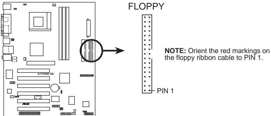
A7V600 SE Floppy Disk Drive Connector
