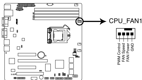
P8B-M CPU FAN connector
