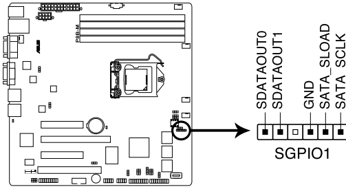
P8B-M SGPIO1 connector
