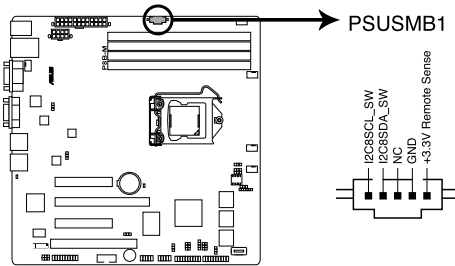
P8B-M Power supply SMBus connector
