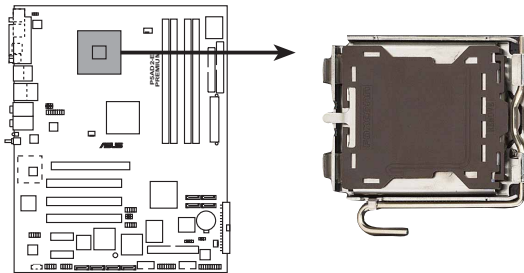
P5A2-E PREMIUM Socket 775
