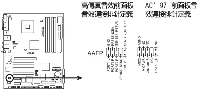
P5AD2-E PREMIUM Analog front panel connector
