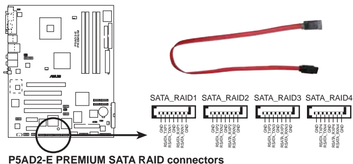
P5AD2-E PREMIUM SATA RAID connectors
