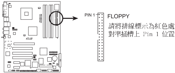
P5AD2-E PREMIUM Floppy disk drive connector
