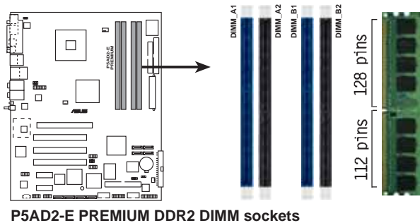
P5AD2-E PREMIUM DDR2 DIMM sockets
