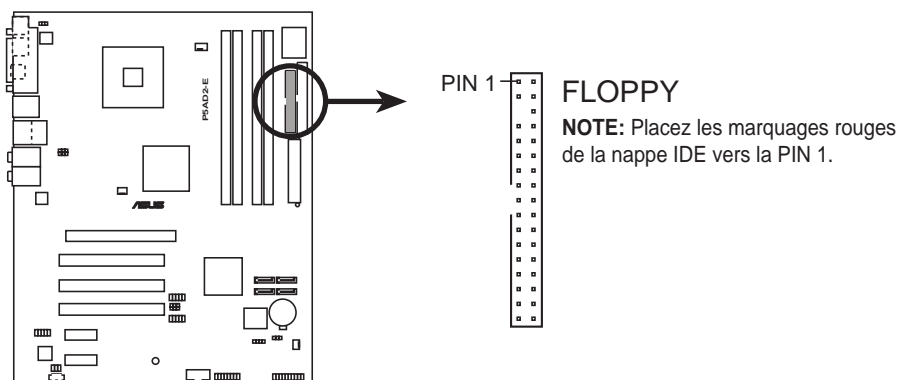
P5AD2-E Floppy disk drive connector
