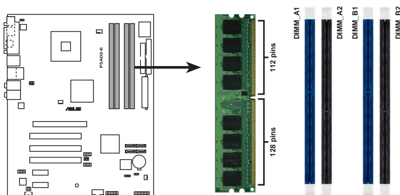
P5AD2-E DDR2 DIMM sockets
