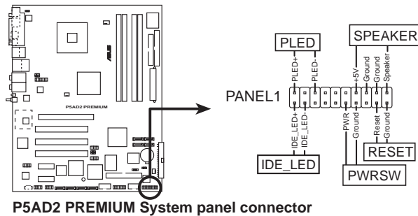
P5AD2 PREMIUM System panel connector
