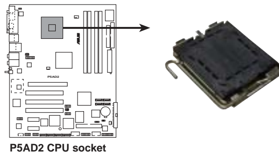
P5AD2 CPU socket
