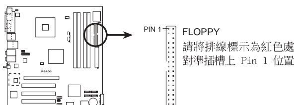
P5AD2 Floppy disk drive connector
