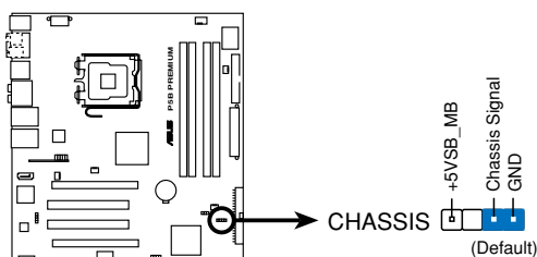
P5B PREMIUM Chassis intrusion connector
