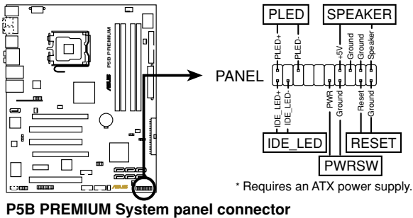
P5B PREMIUM System panel connector
