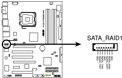
P5B PREMIUM SATA_RAID connector
