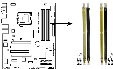
P5B PREMIUM 240-pin DDR2 DIMM sockets
