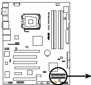
P5B PREMIUM SATA connectors
