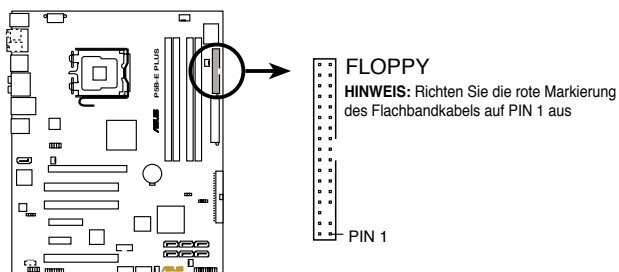
P5B-E PLUS Floppy disk drive connector
