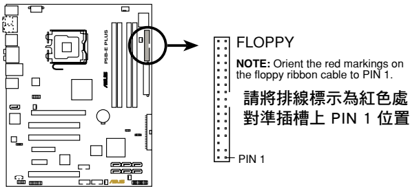
P5B-E PLUS Floppy disk drive connector
