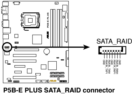
P5B-E PLUS SATA_RAID connector
