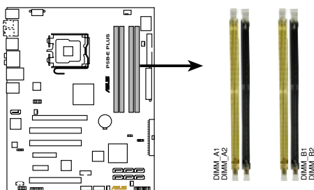
P5B-E PLUS 240-pin DDR2 DIMM sockets
