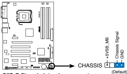
P5B-E Chassis intrusion connector
