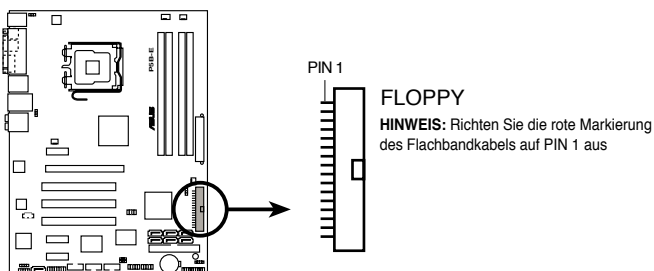
P5B-E Floppy disk drive connector
