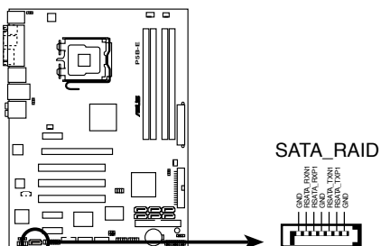
P5B-E SATA_RAID connector
