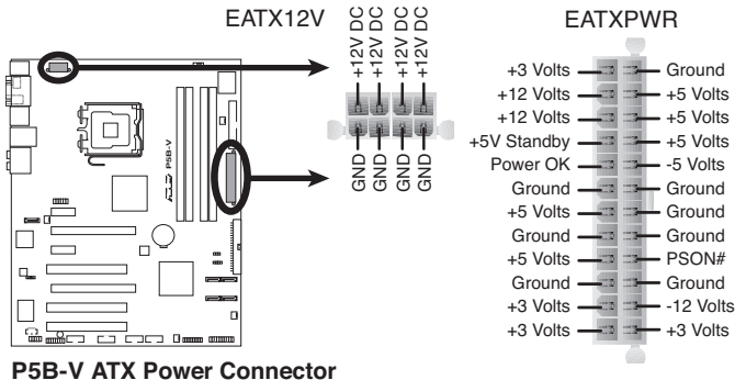
P5B-V ATX Power Connector
