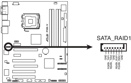
P5B-V SATA RAID Connector
