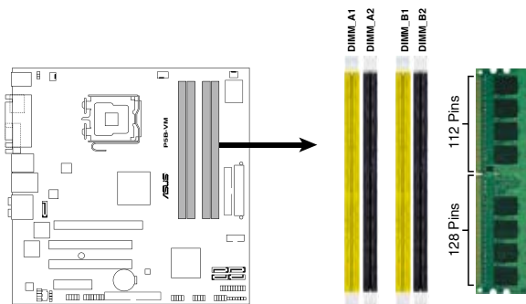
P5B-VM 240-pin DDR2 DIMM Sockets
