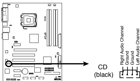
P5B Internal Audio Connector
