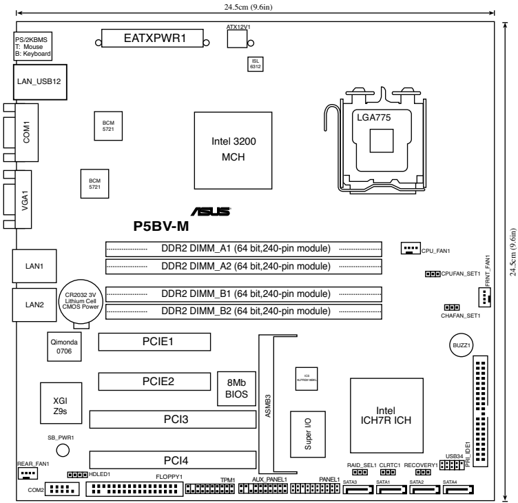
P5BV-M Layout
