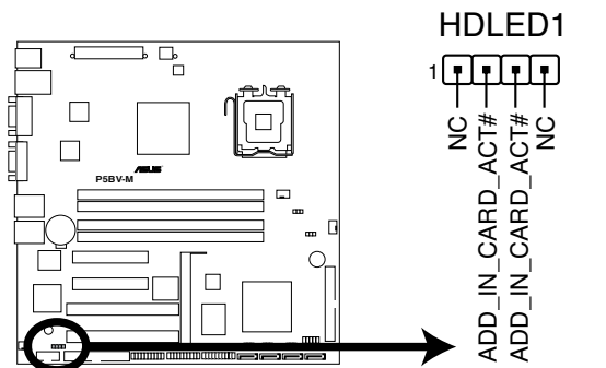
P5BV-M Card Activity LED Connector
