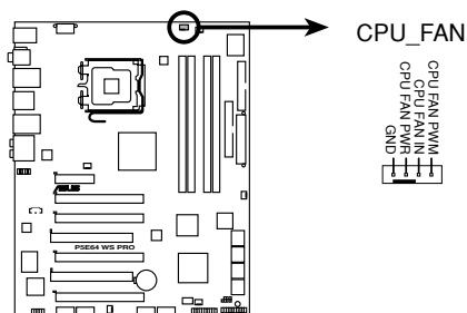
P5E64 WS Professional CPU fan connector
