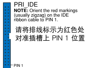
P5E64 WS Professional IDE connector
