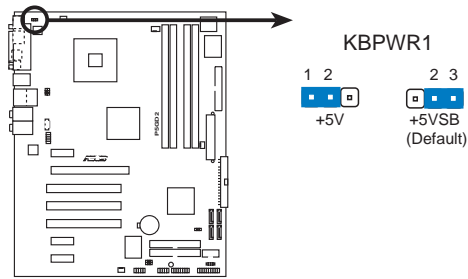
P5GD2 Keyboard power setting
