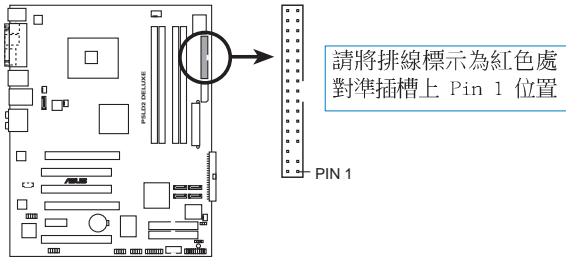
P5LD2 DELUXE Floppy disk drive connector
