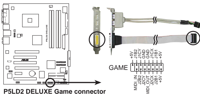
P5LD2 DELUXE Game connector
