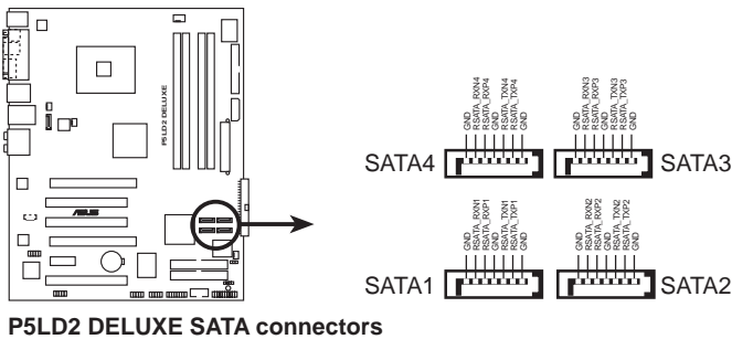
P5LD2 DELUXE SATA connectors
