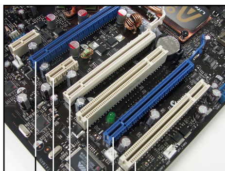
Slot PCI Slot PCI Express x 16 (bleu) Slot PCI Slot PCI Express x 16 (x 8 - blanc) Slot PCI Express x 1 Slot PCI Express x 16 (bleu)
