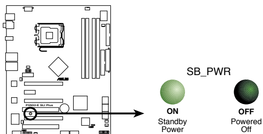
P5N32-E SLI Plus Onboard LED
