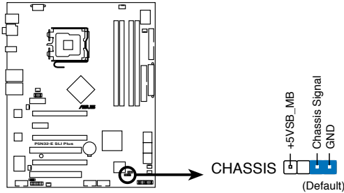
P5N32-E SLI Plus Chassis intrusion connector
