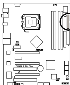
P5N32-E SLI Plus Floppy disk drive connector
