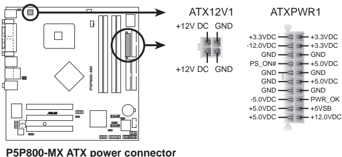
P5P800-MX ATX power connector
