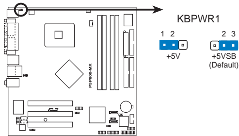
P5P800-MX Keyboard power setting
