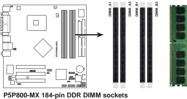
P5P800-MX 184-pin DDR DIMM sockets
