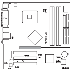
P5P800-VM Accelerated Graphics Port (AGP)
