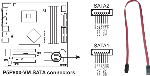
P5P800-VM SATA connectors
