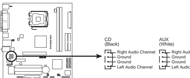
P5V800-MX Internal audio connectors
