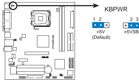
P5V800-MX Keyboard power setting
