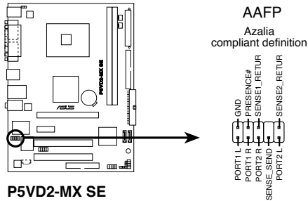
P5VD2-MX SE Analog Front Panel Connector
