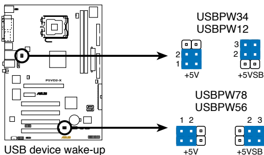
USB device wake-up
