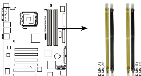
P5W64 WS PRO 240-pin DDR2 DIMM sockets
