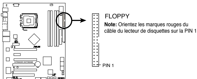
STRIKER EXTREME Floppy disk drive connector
