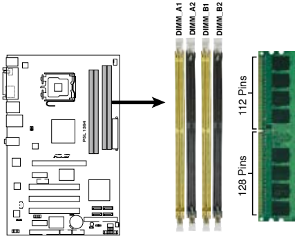
P5L 1394 240-pin DDR2 DIMM Sockets
