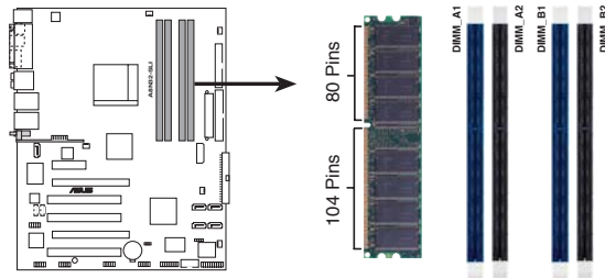
A8N32-SLI 184-pin DDR DIMM sockets
