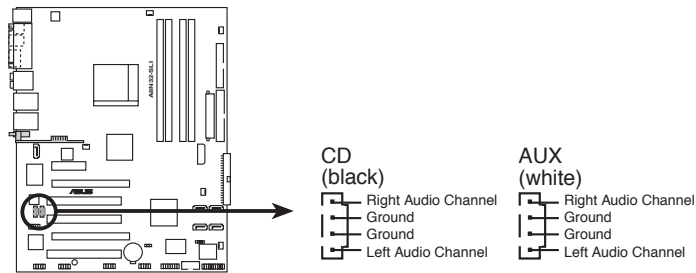
A8N32-SLI Internal audio connectors
