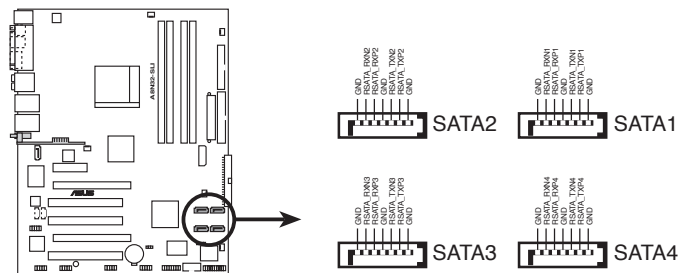
A8N32-SLI SATA connectors
