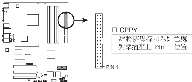
A8N5X Floppy disk drive connector
