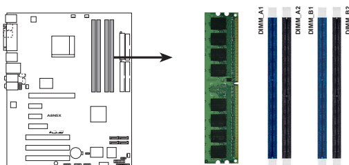
A8N5X 240-pin DDR2 DIMM sockets
