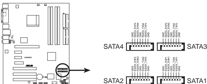
A8N5X SATA connectors
