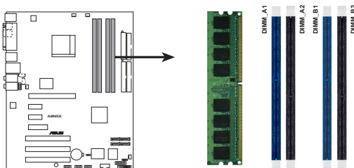
A8N5X 184-pin DDR DIMM sockets
