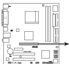
A8V-MX Accelerated Graphics Port (AGP)
