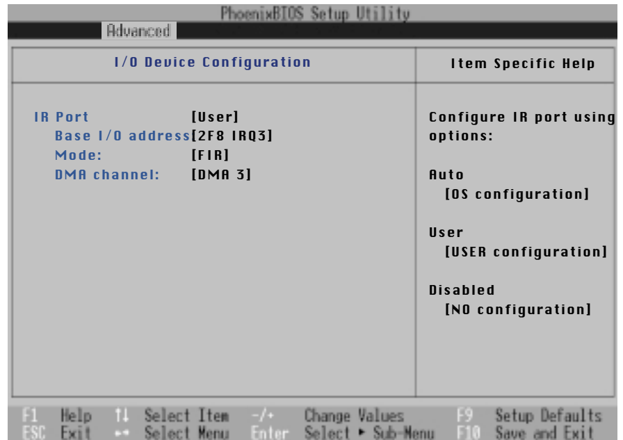
圖6-6 I/O Device Configuration次菜單
