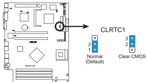
PSCH-LR Clear RTC RAM
