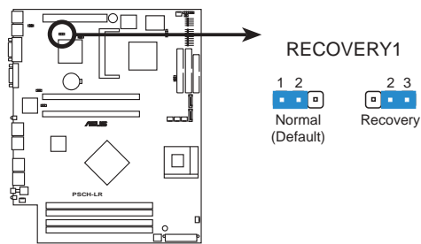
PSCH-LR RECOVERY Setting
