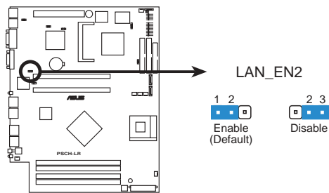
PSCH-LR LAN_EN2 Setting
