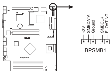
PSCH-LR SMB Connector
