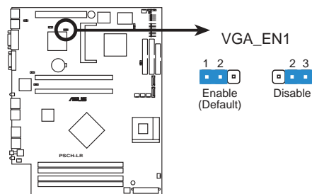
PSCH-LR VGA Jumper Setting
