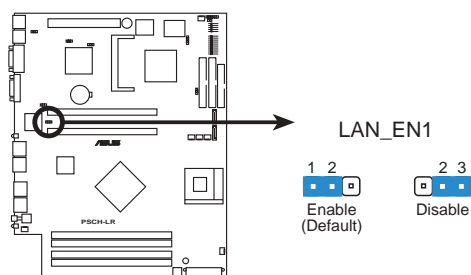
PSCH-LR LAN_EN1 Setting
