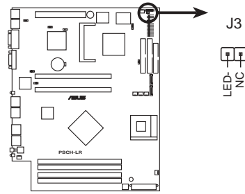
PSCH-LR J3 Connector
