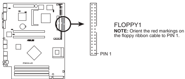
PSCH-LR Floppy Disk Drive Connector
