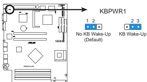
PSCH-LR Keyboard Power Setting
