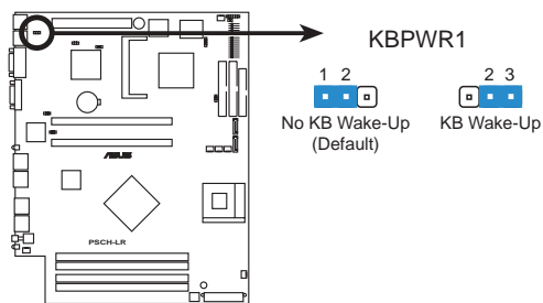
PSCH-LR Keyboard Power Setting
