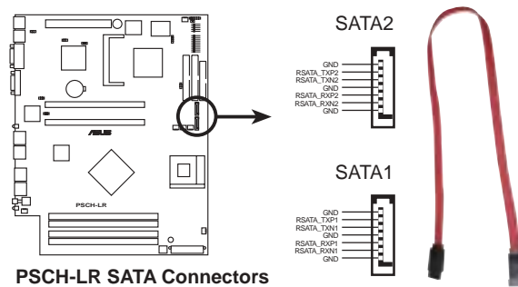
PSCH-LR SATA Connectors
