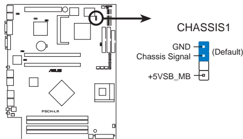
PSCH-LR Chassis Alarm Lead
