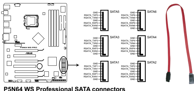
P5N64 WS Professional SATA connectors
