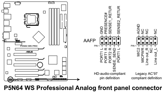
P5N64 WS Professional Analog front panel connector
