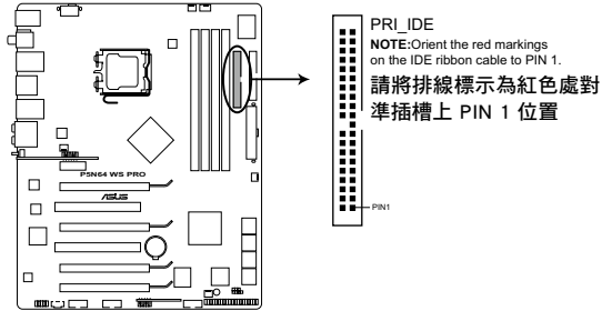
P5N64 WS Professional IDE connector
