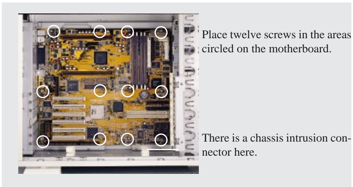
Installed motherboard
