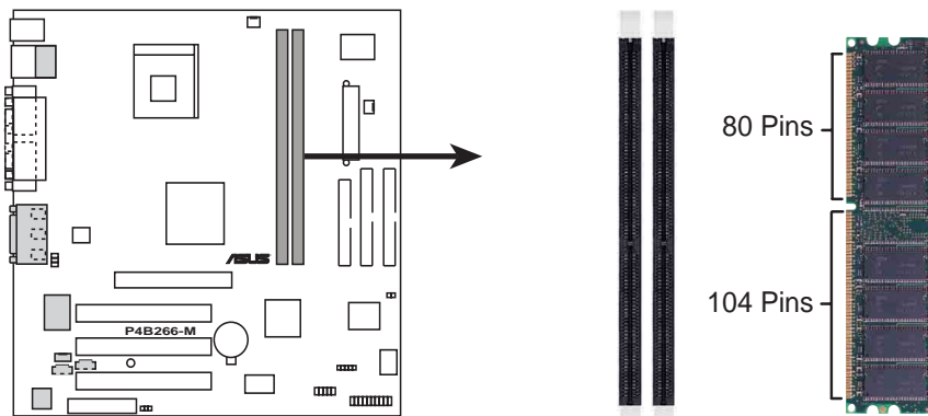
P4B266-M 184-Pin DDR DIMM Sockets
