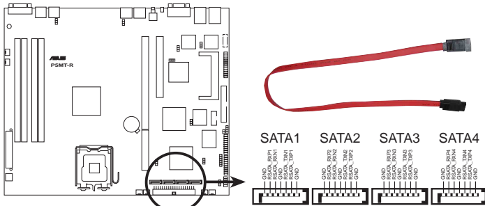
P5MT-R SATA connectors
