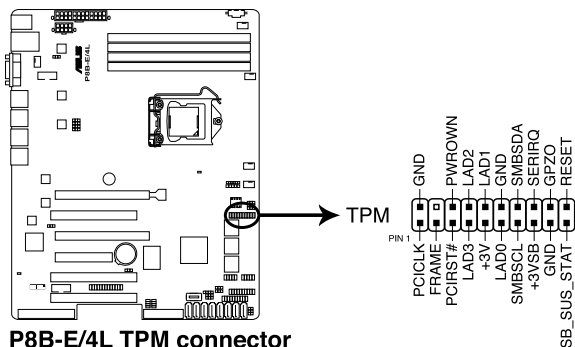
P8B-E/4L TPM connector
