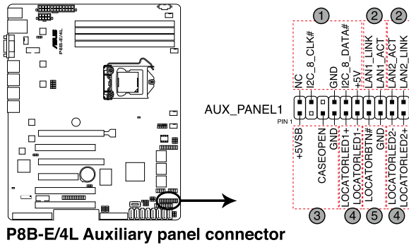
P8B-E/4L Auxiliary panel connector
